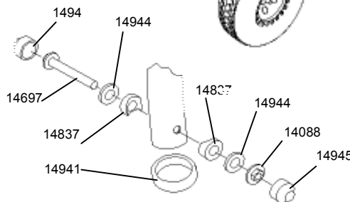
Fig 3 – Connection Detail
