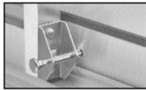
EDGE OF FIXED DOOR (OUTSIDE SLIDING DOOR)
