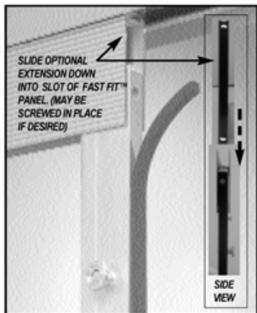
FIG. 3 - PANEL BUMPER SEAL
