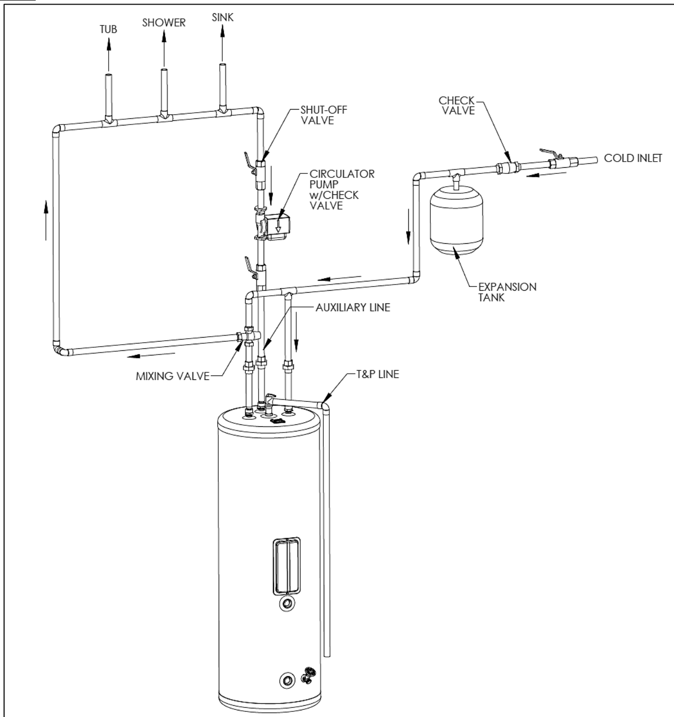
Figure 4 – Typical Expansion Tank Application with Auxiliary Line – LP-451-A
