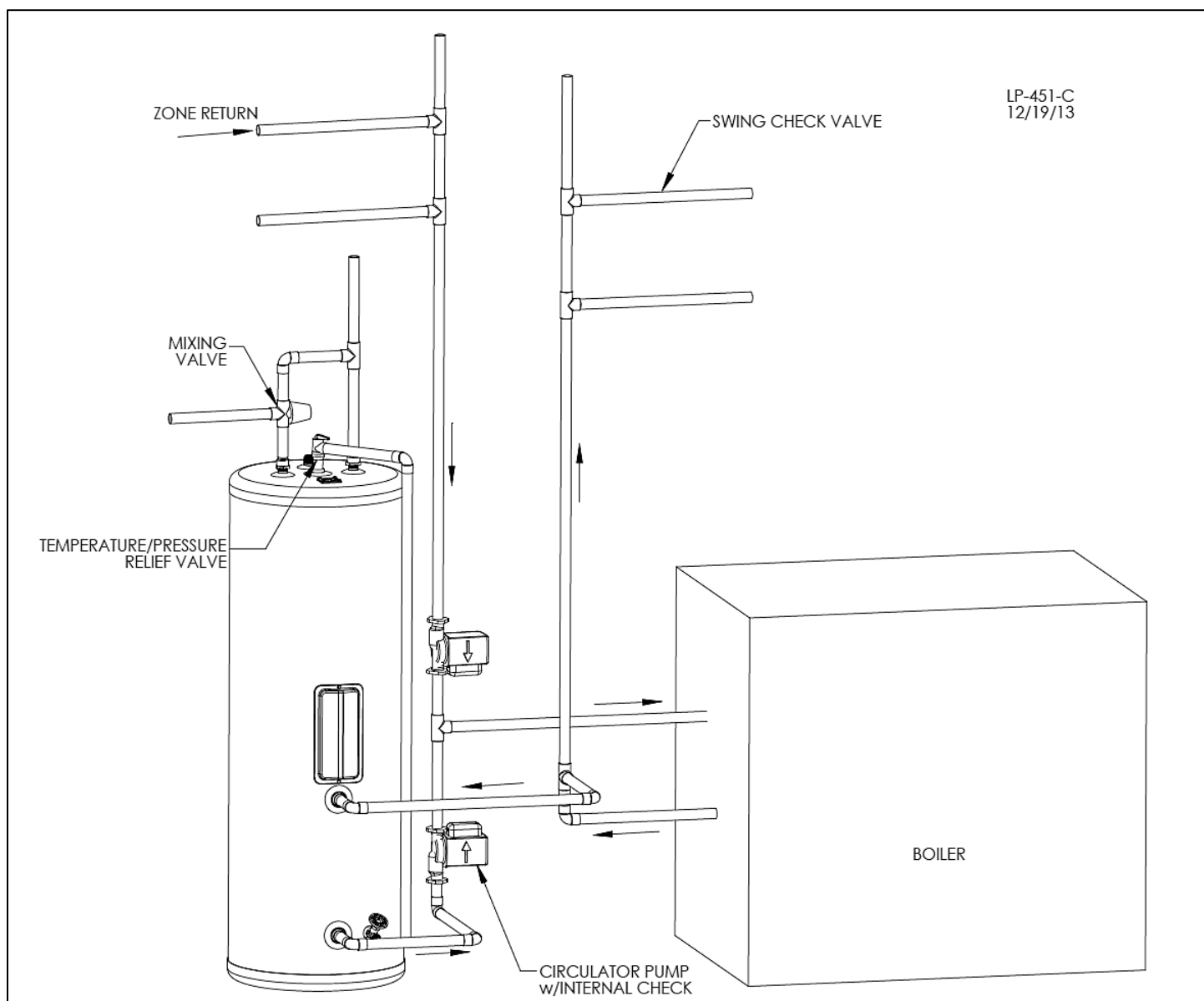
Figure 6 – Zoning with Circulators
