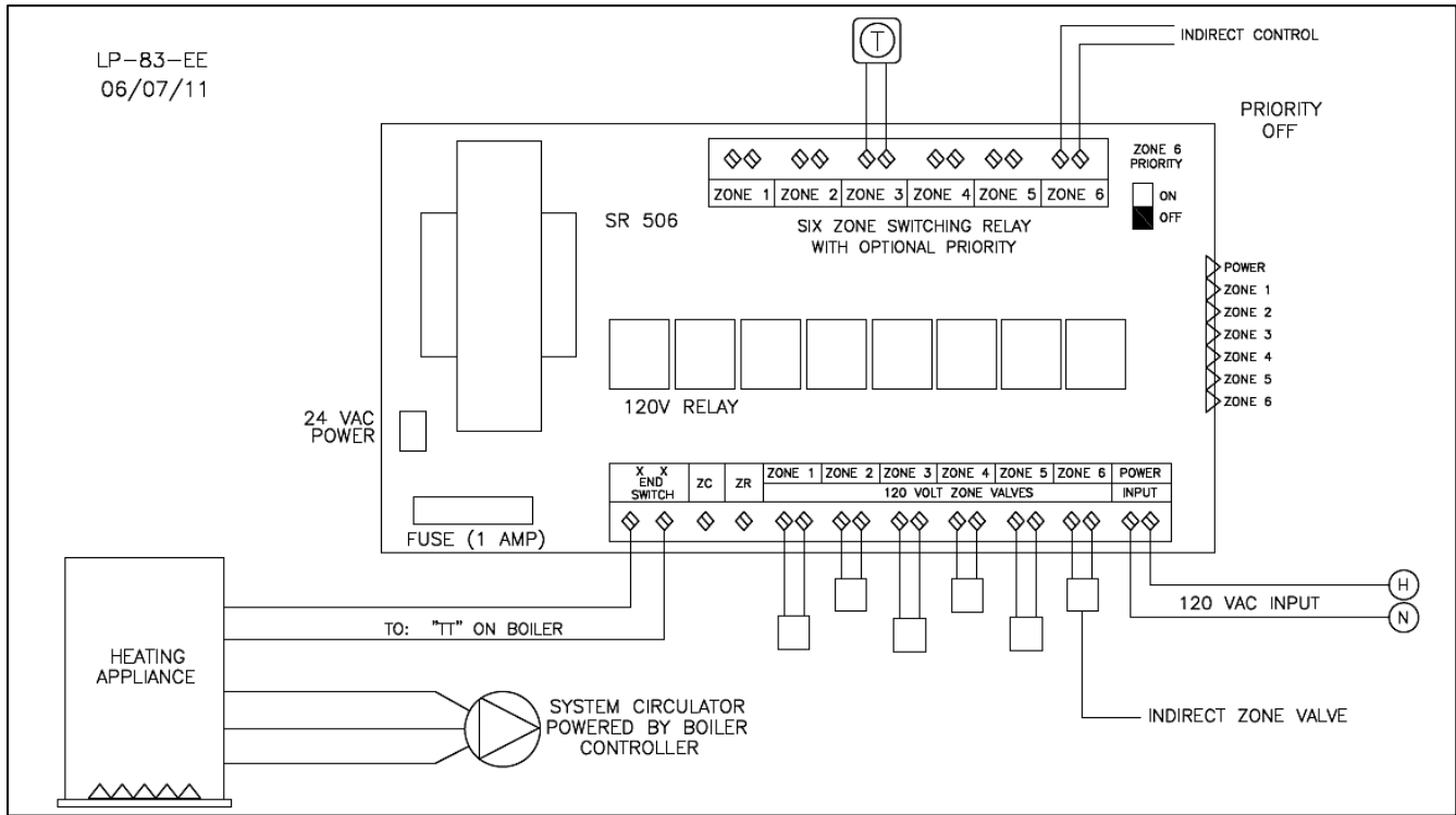
Figure 9 – Wiring with Zone Valves
