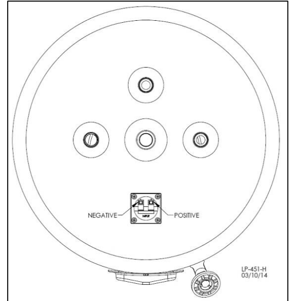
Figure 7 – Thermostat Connection
