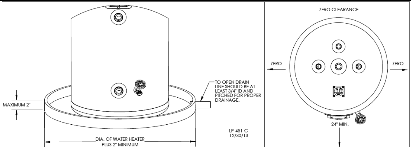
Figure 2 – Recommended Service Clearances
