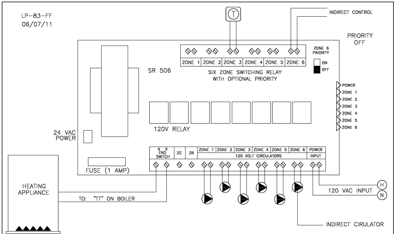
Figure 8 – Wiring with Circulators
