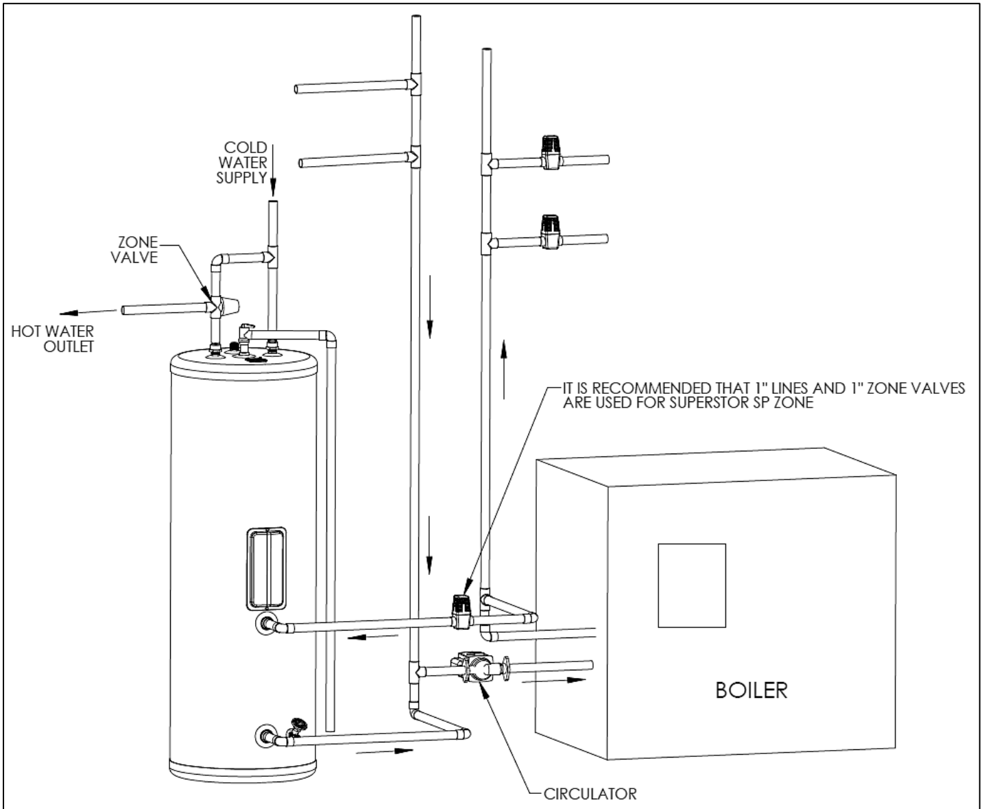
Figure 5 – Zoning with Zone Valves – LP-451-B
