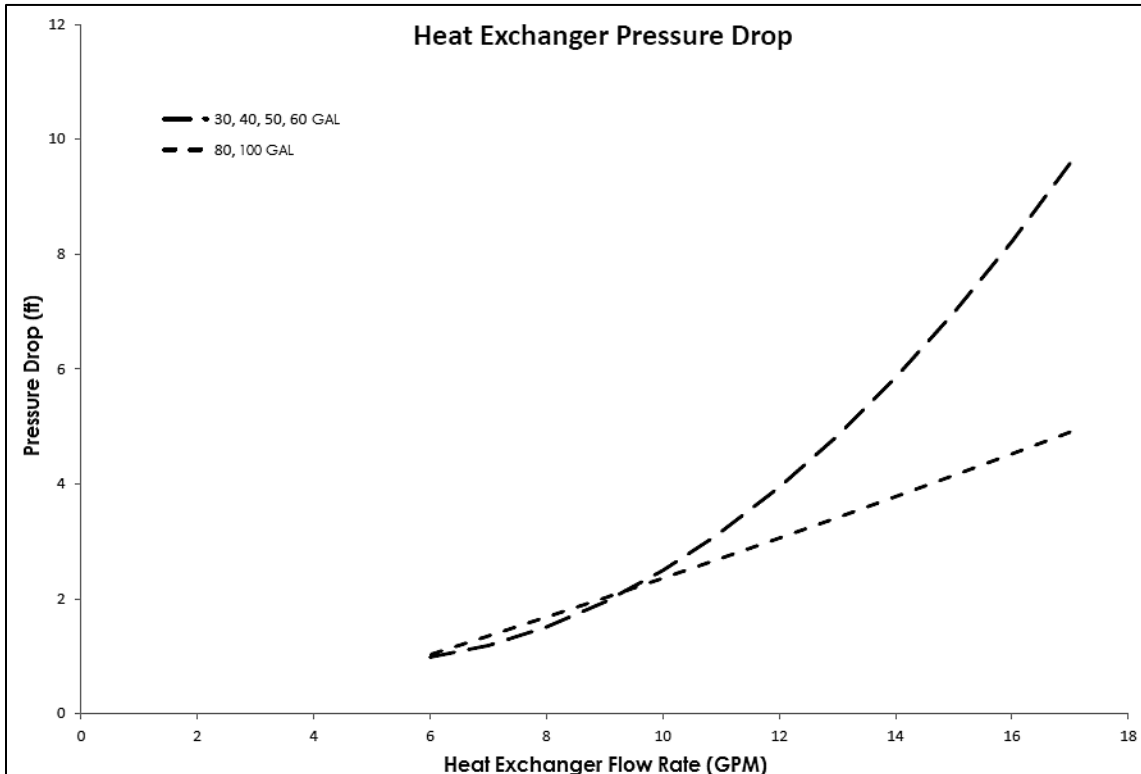
Figure 3 – Pressure Drop Through the Heat Exchanger
