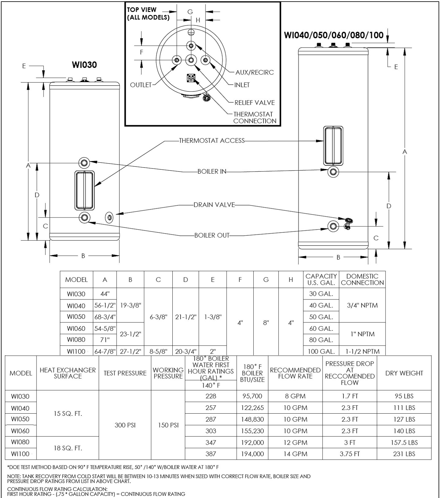
Figure 1 – Specifications and Dimensions
