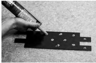
Method 2 - Using high-quality polyurethane construction adhesive
