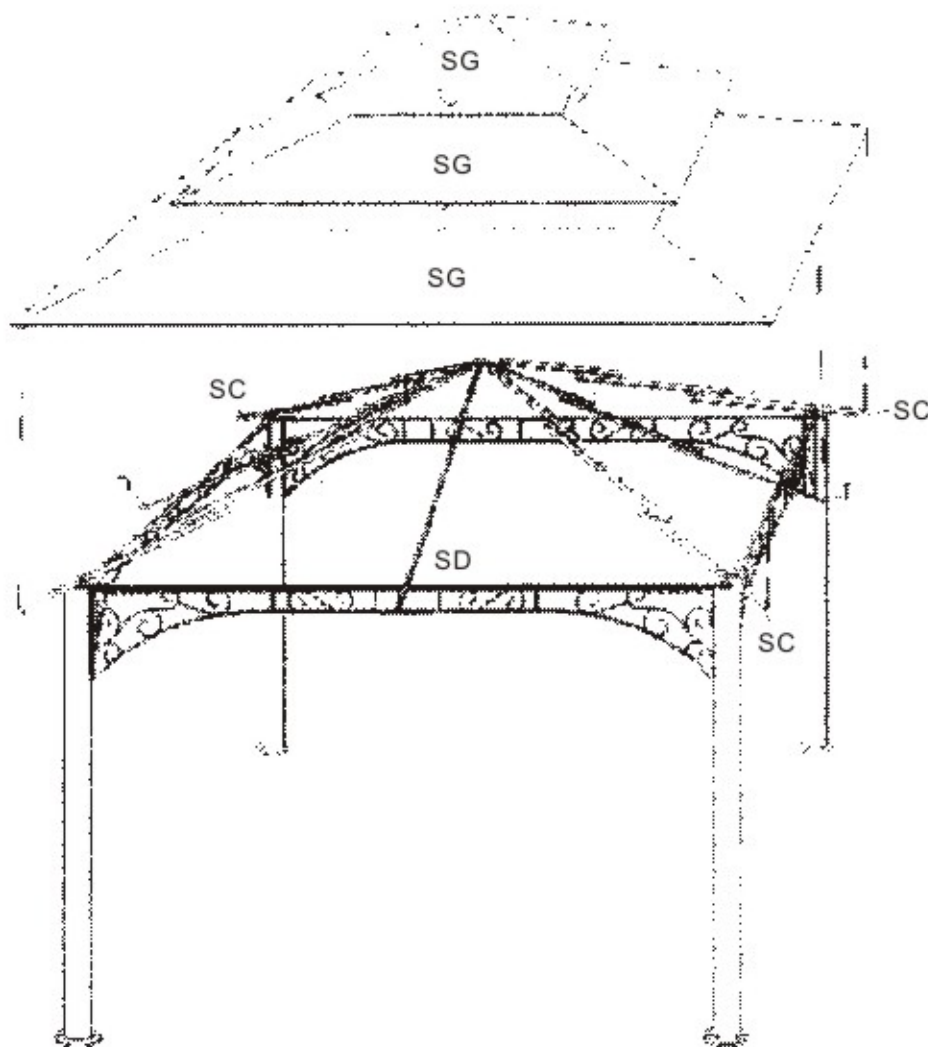
Figure 4 Cover Assembly
