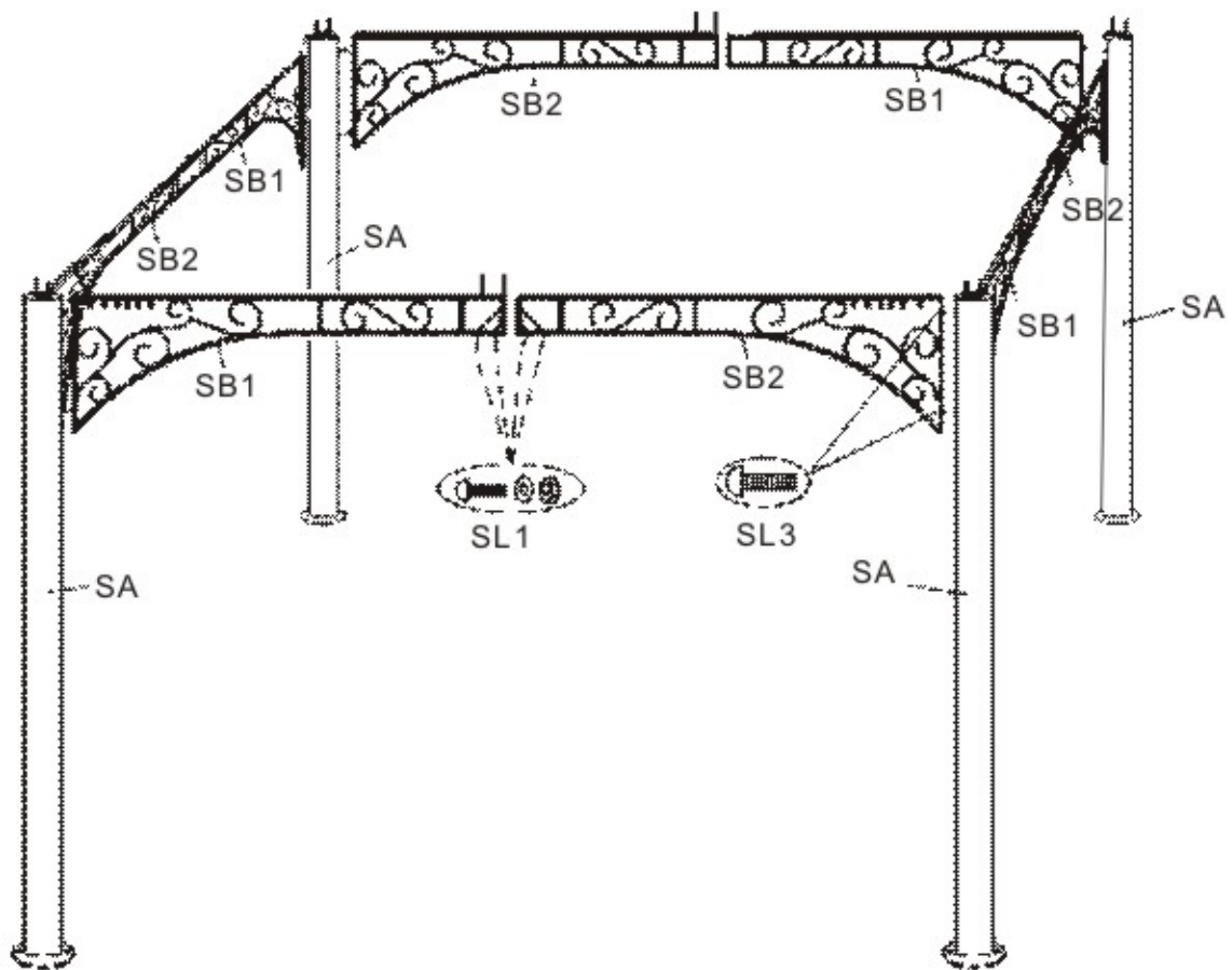
Figure 1 Frame Assembly
