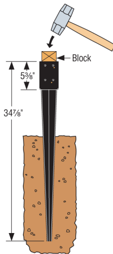
E-Z Spike™ (FPBS44)
