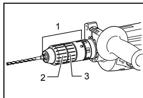
1. Quick change drill chuck 2. Sleeve 3. Ring
