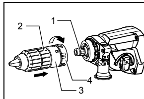
1. Spindle 2. Change drill chuck 3. Change cover 4. Change cover line
