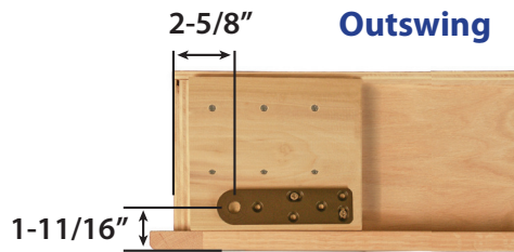
Outswing
