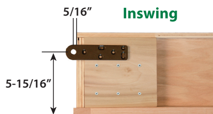
Inswing
