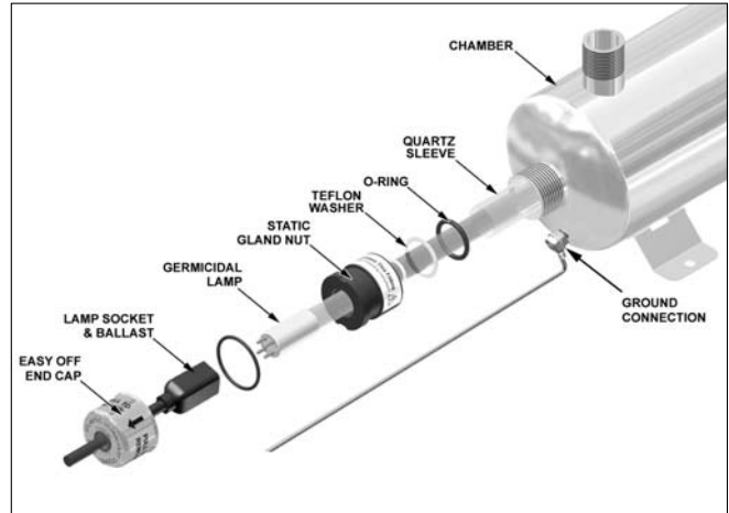
Figure 10 - Quartz Sleeve Cleaning or Replacement MIN-6 230v 50/60Hz (ballast no. 10-0504A)
