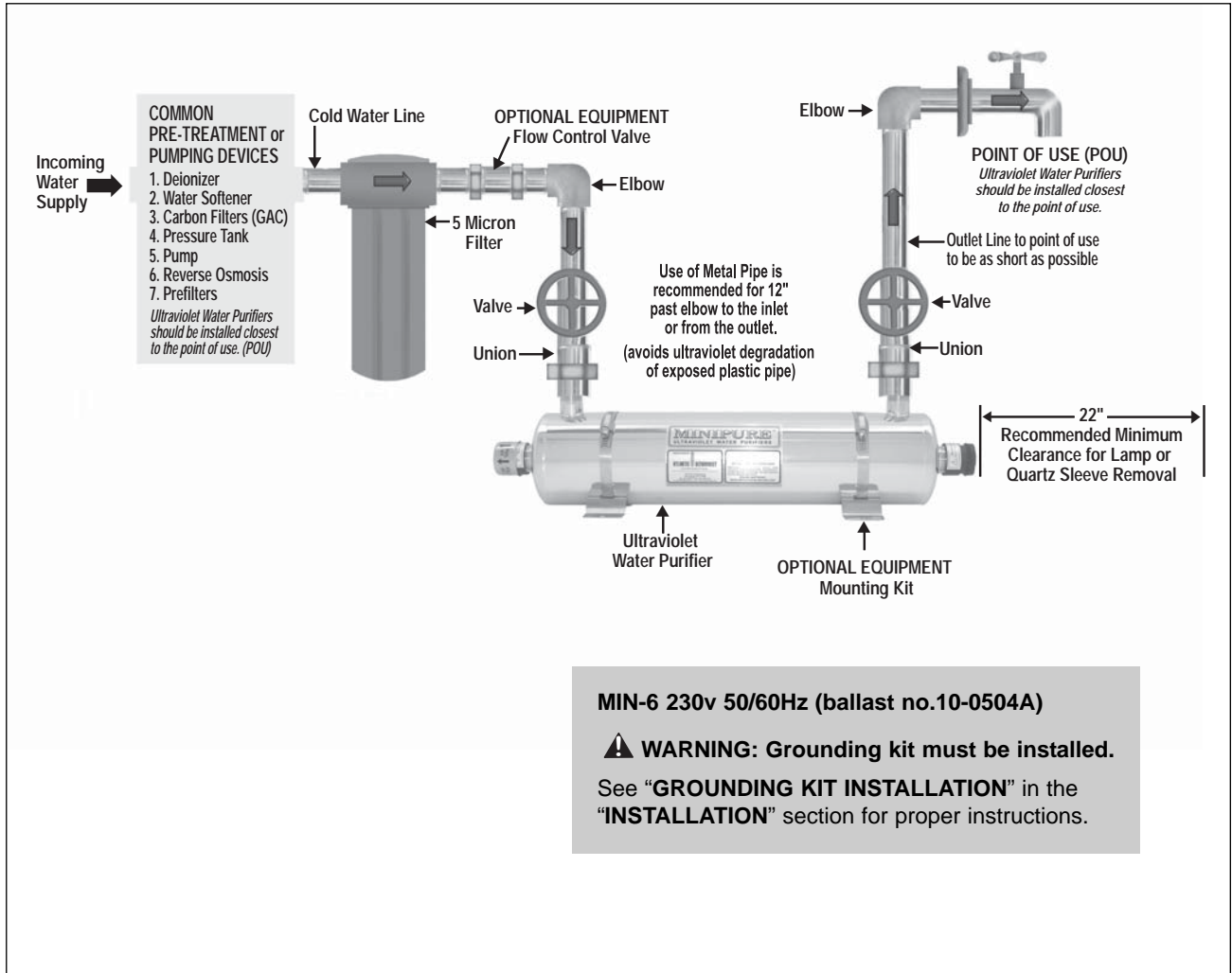
Figure 3 - Recommended Installation
