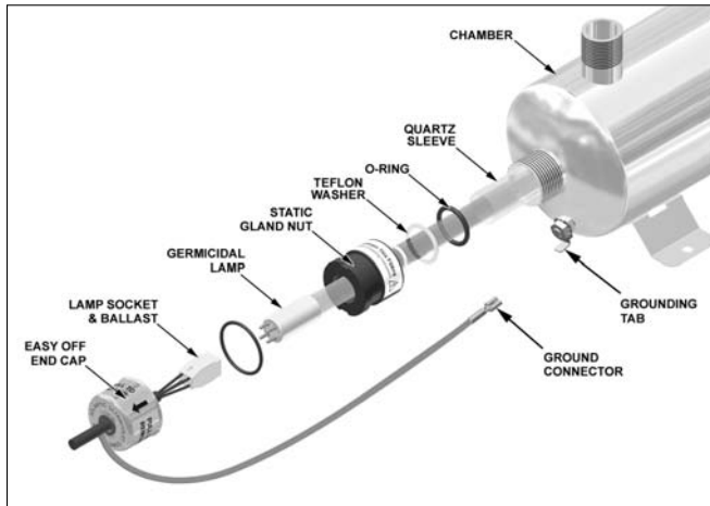
Figure 9 - Quartz Sleeve Cleaning or Replacement MIN-6 120v 50/60Hz (ballast no. 10-0015B)
