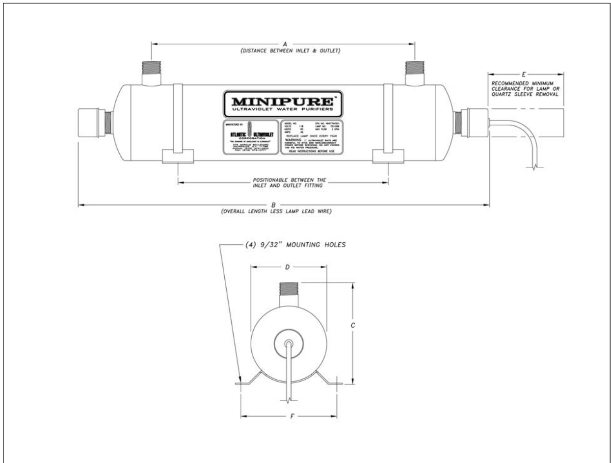
Figure 2 - MIN-6 Dimensional Drawing
