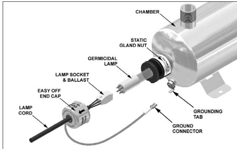
Figure 7 - Lamp Replacement for Model MIN-6 120v 50/60Hz (ballast no. 10-0015B)
