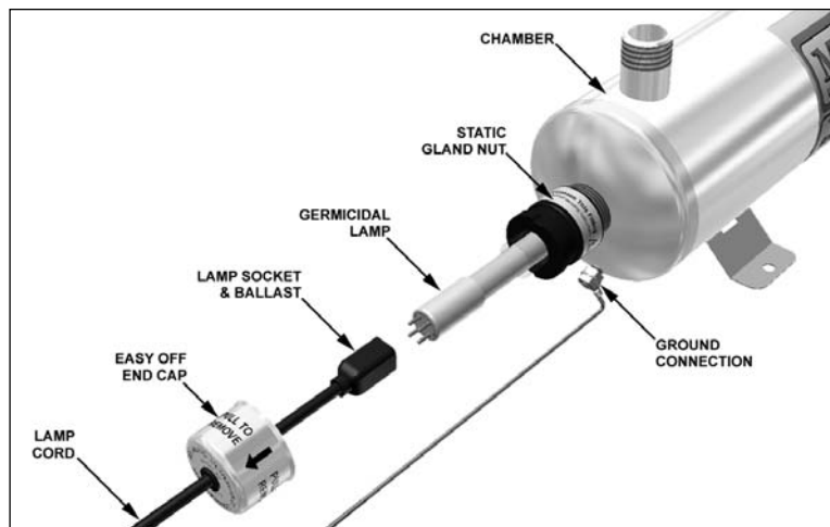
Figure 5 - 230v 50/60Hz (ballast no. 10-0504A)
