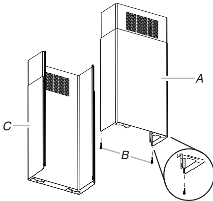
A. Upper and lower duct cover assembled - (front placement) B. Plastic clips (2) (long end for front placement) C. Upper and lower duct covers assembled - (rear placement)
